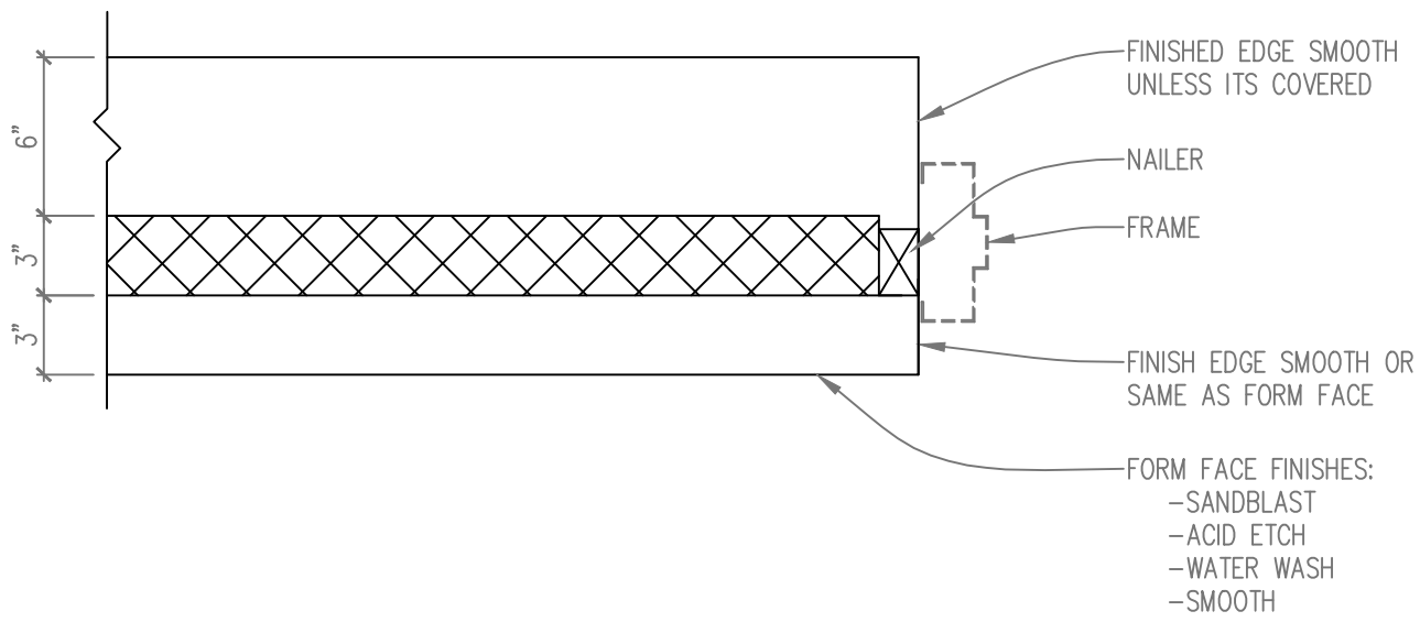
- FINISHES @ OPNG DETAIL SCALE: 1 1/2" = 1'-0"
