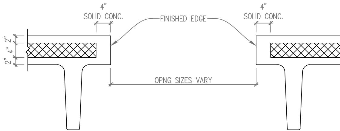
— OPENING W/ SOLID CONC. (DETAIL) SCALE: 3/4" = 1'-0"
