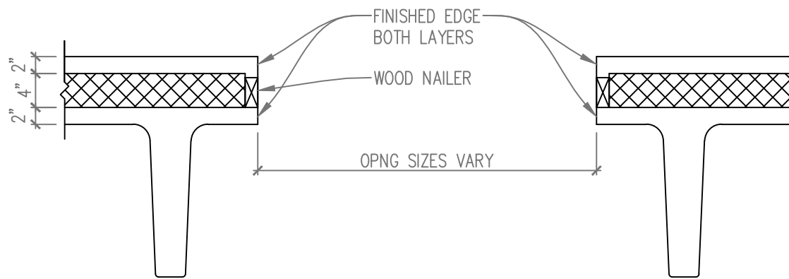
— OPENING W/ WOOD NAILER DETAIL SCALE: 3/4" = 1'-0"
