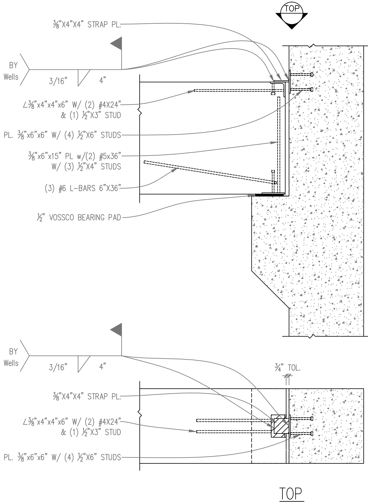
- RECTANGULAR BEAM BEARING ON COLUMN HAUNCH DETAIL SCALE: \frac{3}{4} " = 1'-0"
