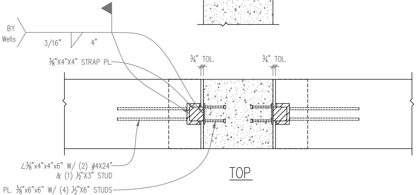
— TWO RECTANGULAR BEAMS BEARING ON COLUMN HAUNCHES DETAIL SCALE: 3/4" = 1'-0"
